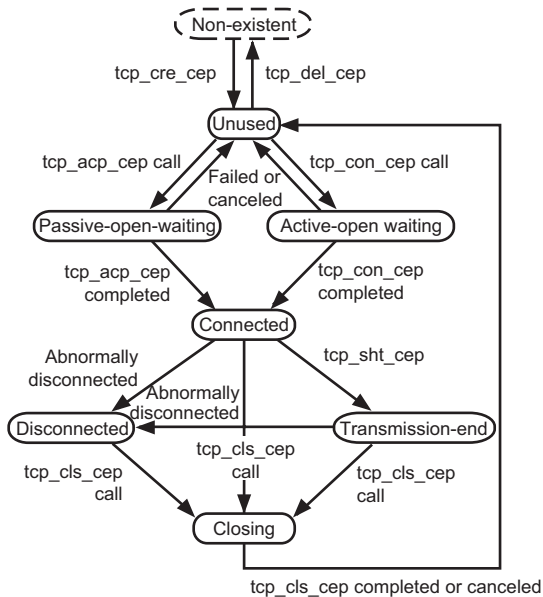
Figure 1. State Transition of TCP Communication End Point
